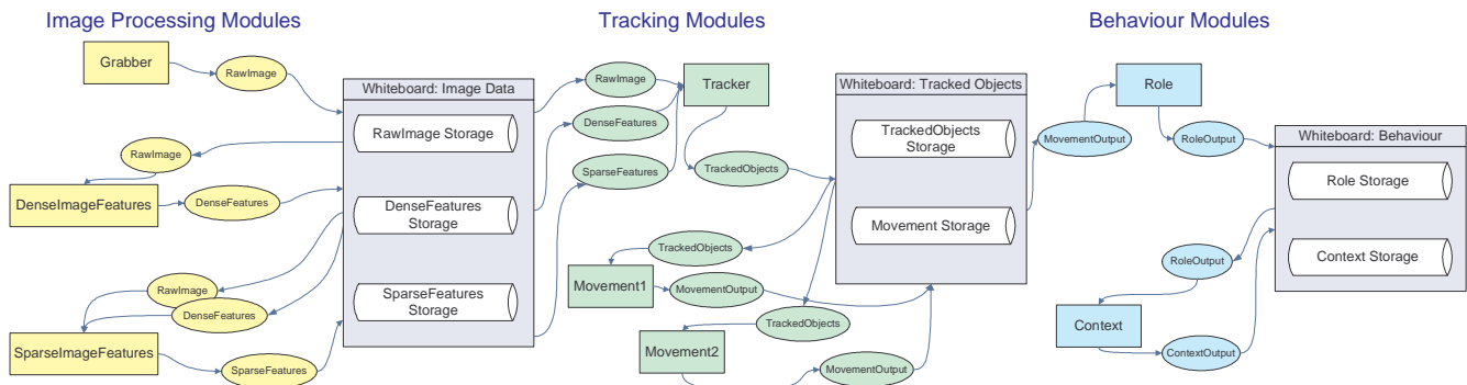
Fig. 2. The system data and processing flowchart from Psyclone. (Data structures are listed twice, once for input and once for output.)
