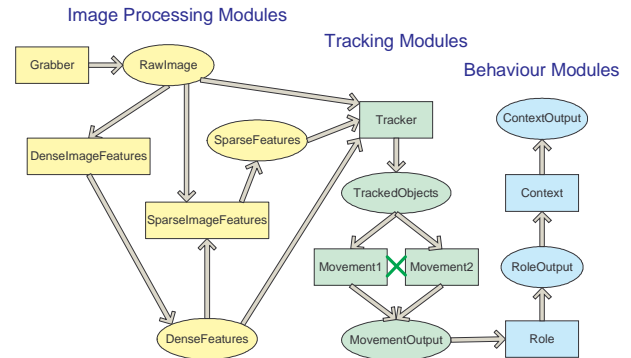
Fig. 1. The system data and processing flowchart from CAVIAR
