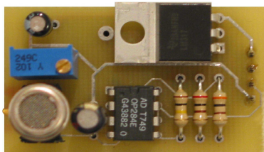
Figure 3-2: Ground-level Ozone Detector
