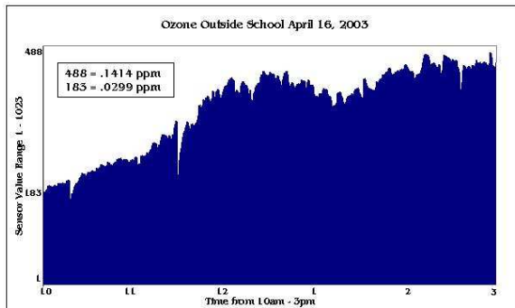
Figure 4-1: Ozone Trend Outdoors
