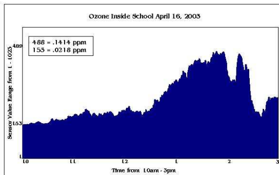
Figure 4-2: Ozone Trend Indoors
