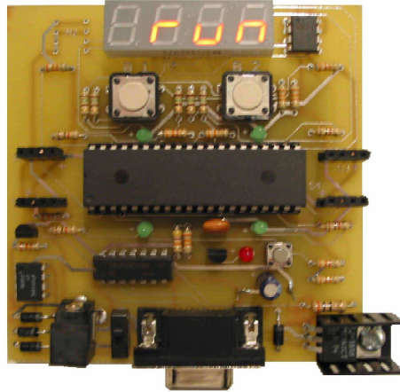
Figure 3-1: Programmable Sensing Board
