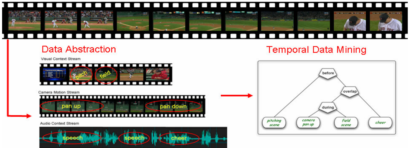
Figure 1. Temporal feature induction operates by first abstracting the raw video into parallel streams corresponding to visual context, camera motion, and audio context features. Temporal data mining then discovers patterns in the streams.
