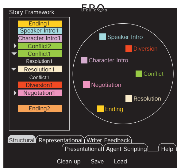
Figure 3 An Agent Story as seen through the structural environment screen; story framework is built by dragging primitives from the circle and dropping them into the story framework retangle
